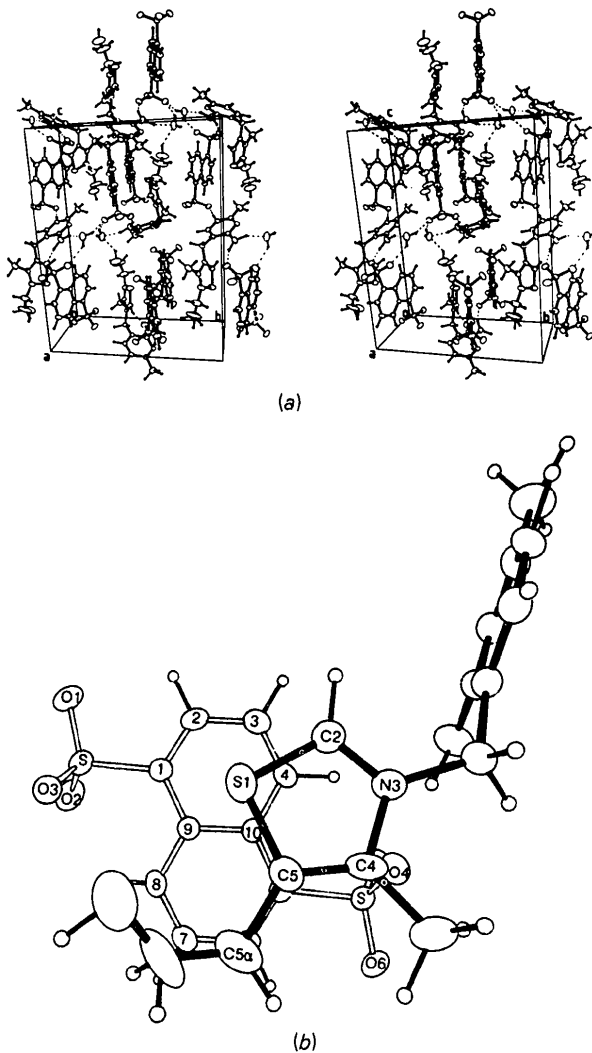
Fig. 2. (a) Stereoscopic view (ORTEP, Johnson, 1976) of the crystal packing. Dashed lines indicate the hydrogen bonds. (b) Perspective view (normal to the naphthalene ring) showing the partial ring stacking interaction. Thermal ellipsoids are drawn at 50% probability.
